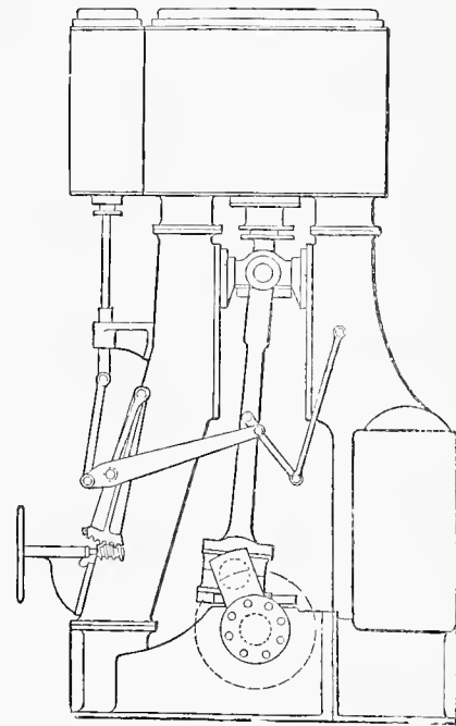
JOY'S VALVE GEAR.
